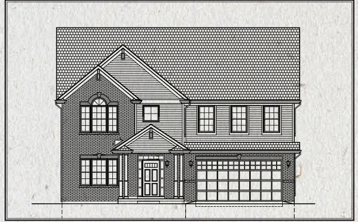
Elevation C
